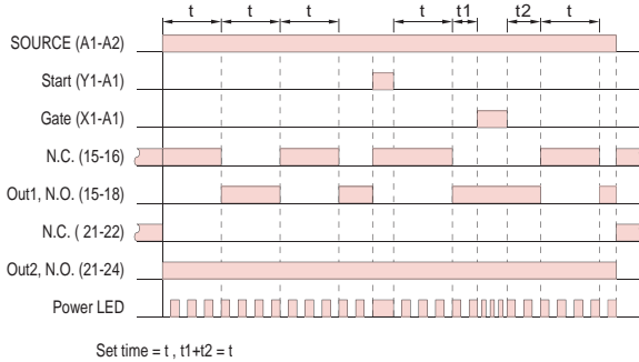
输出模式B3:闪烁反动作(ON先计时)
